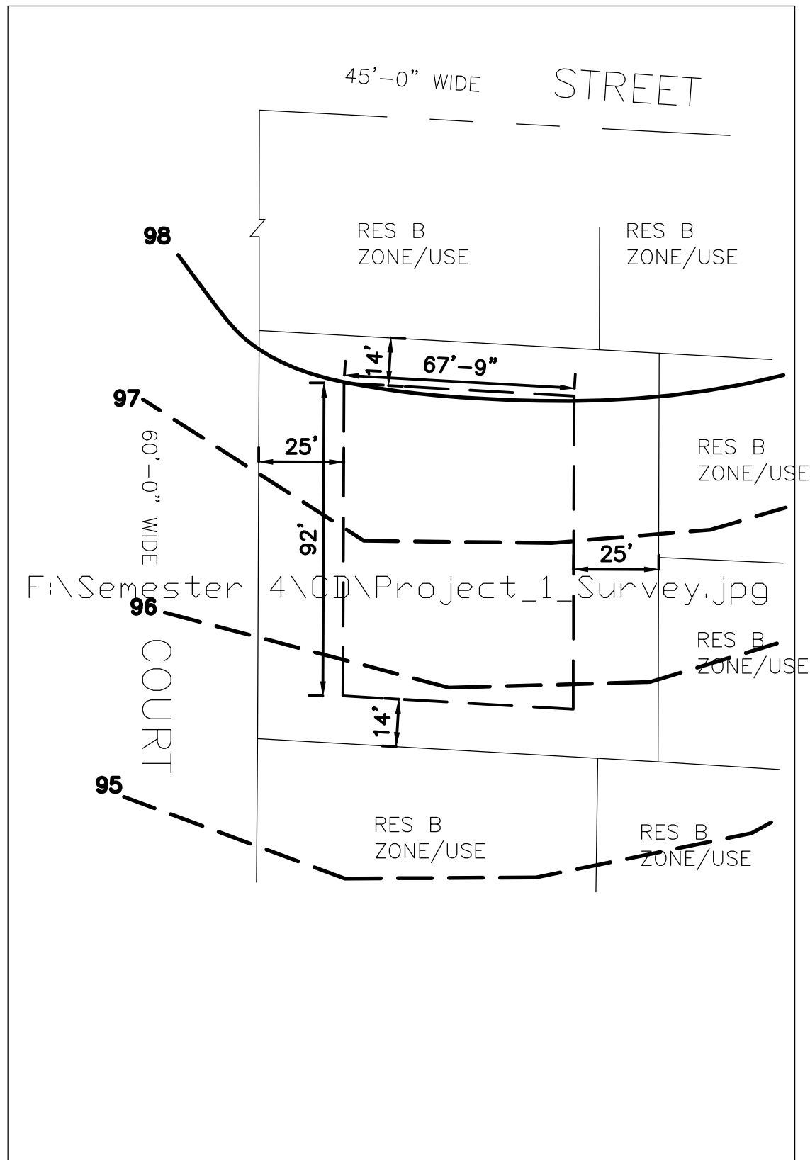
A 002 SITE PLAN SCALE: 1" = 40'
